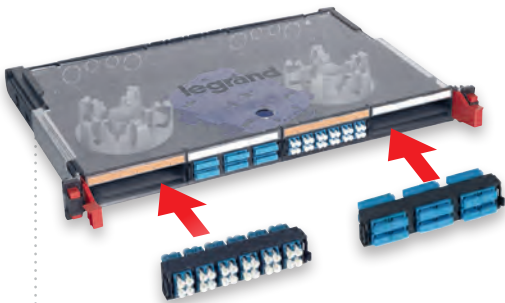
Modular panels
